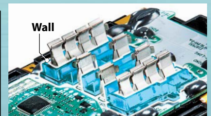
Terminal short-circuit prevention structure The protection wall is provided between terminals against water and dust.
